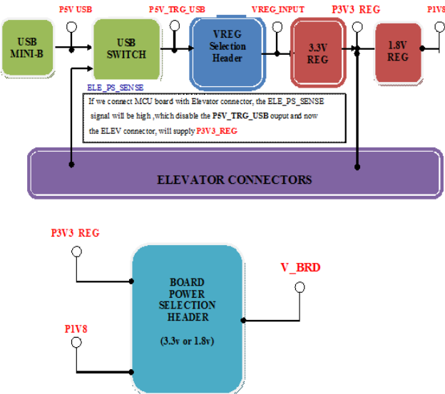
Power Flow
