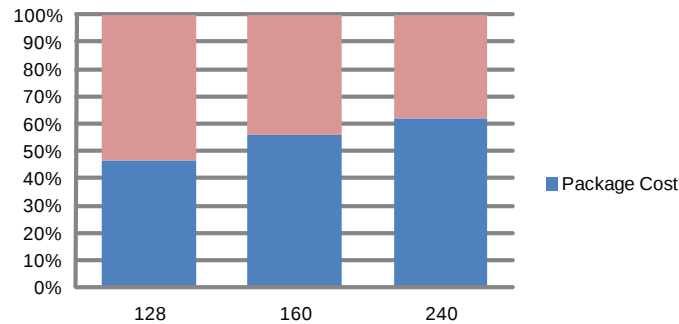
Fig 7. Share of package cost on total display driver cost as function of total number of display elements
