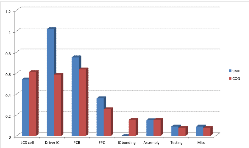
Fig 14. Normalized COG and SMD cost share structure
