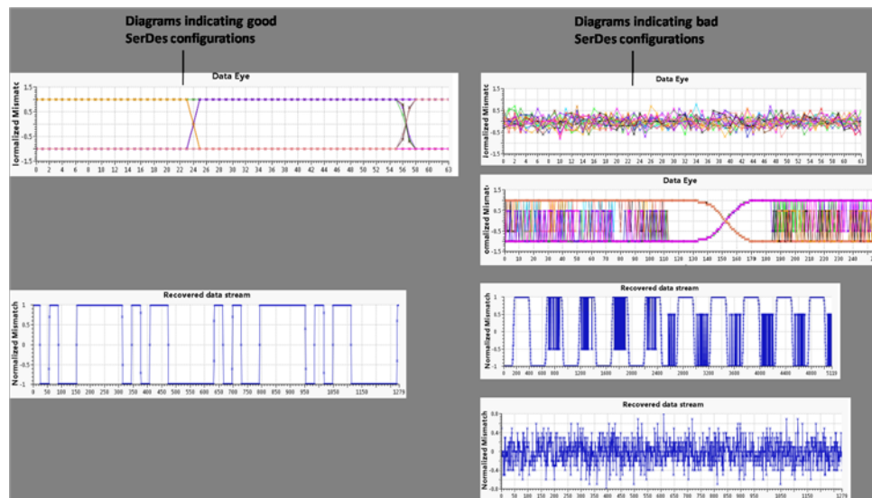
Figure 22. Good versus bad SerDes configuration indicator diagrams
