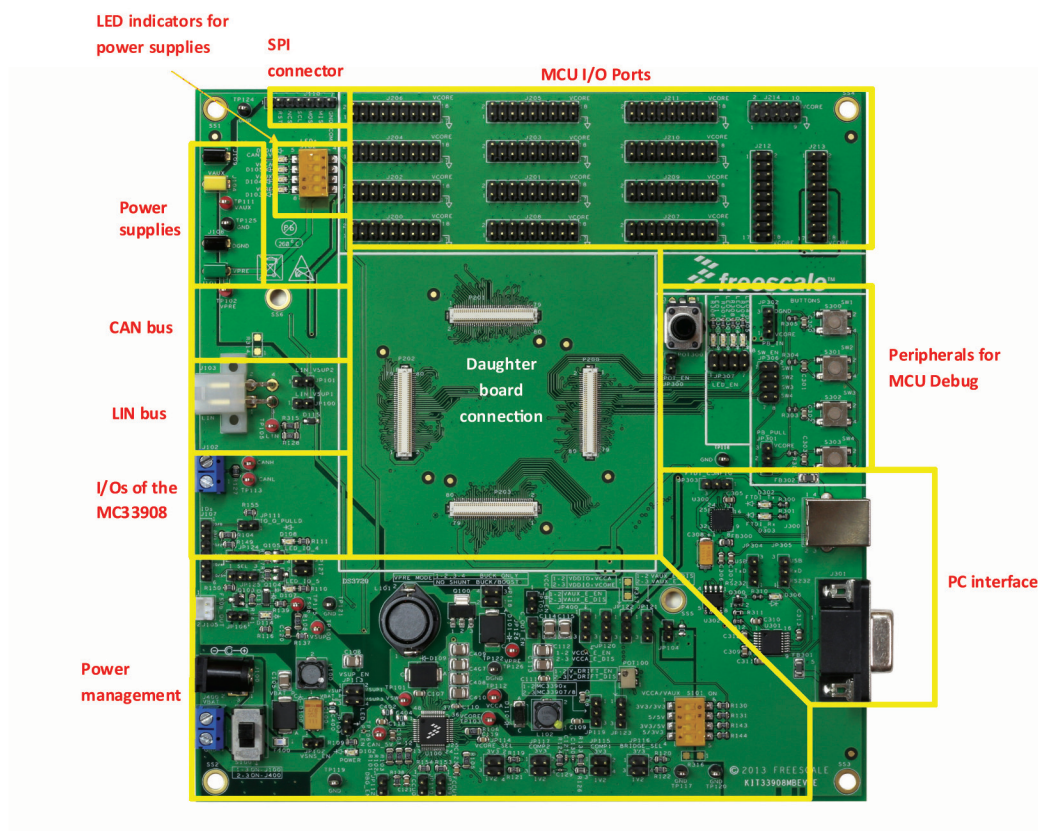
Figure 4. The KIT33908MBEVBE Enhanced Evaluation Board
