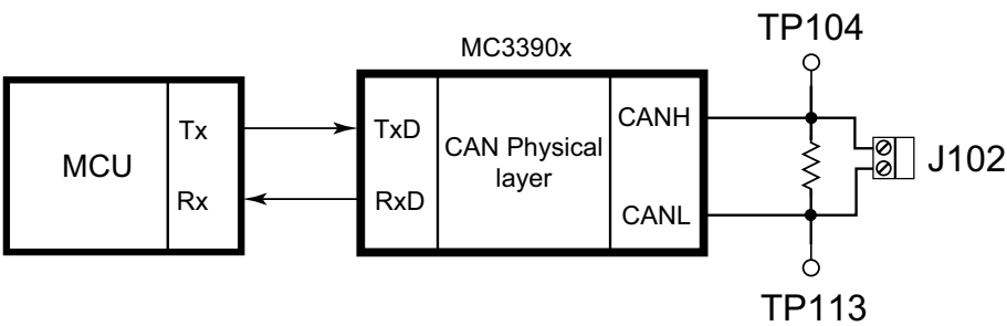
Figure 9. CAN Interface
