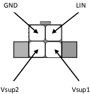
Figure 10. LIN Connector
