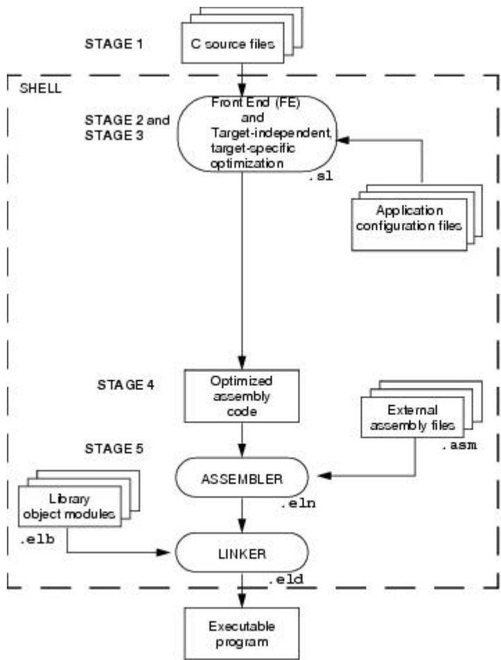
Figure 3-1. Compilation stages
