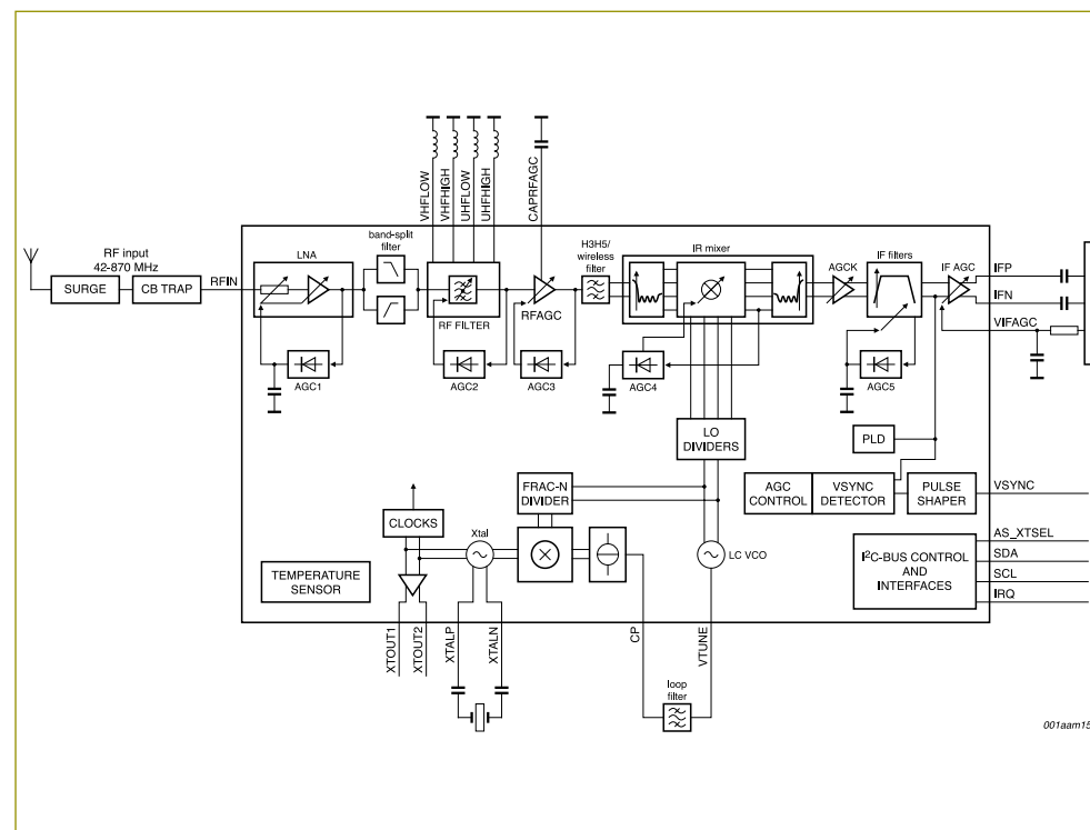
TDA18273 block diagram
