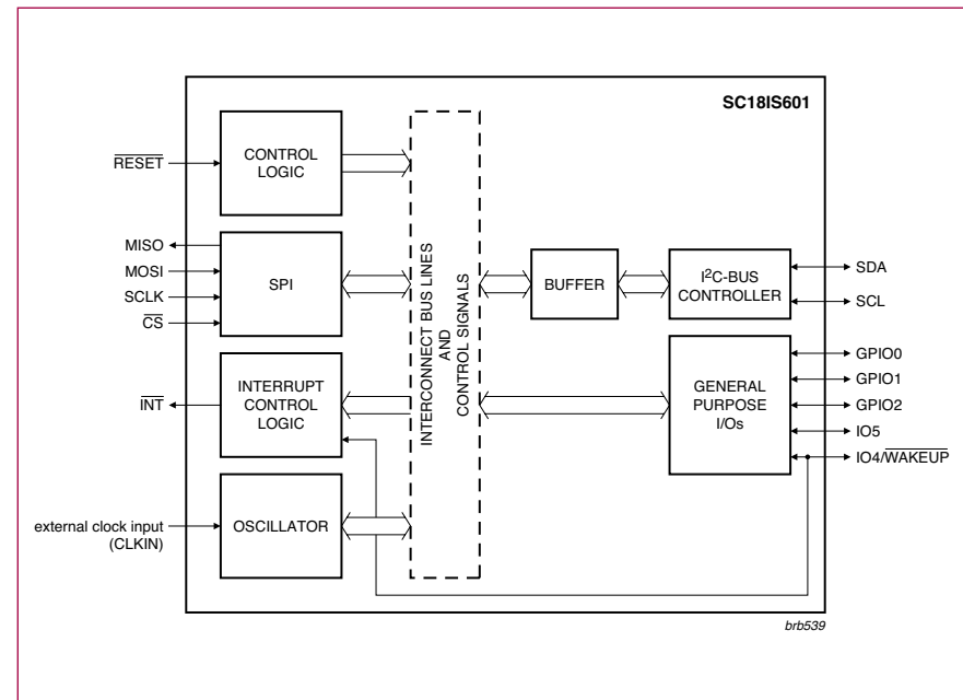
SC18IS601 block diagram
