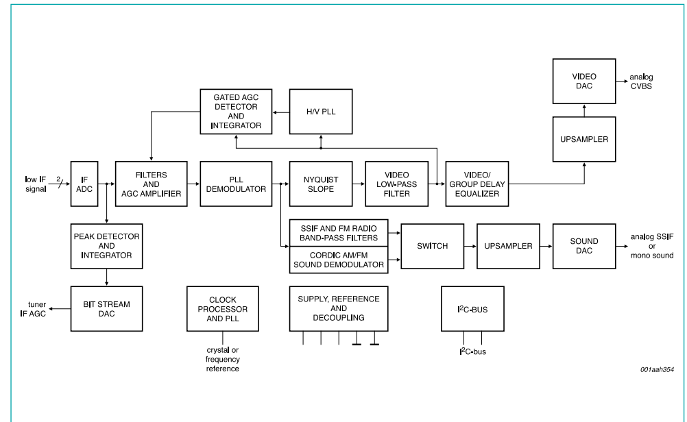
TDA8296 functional diagram
