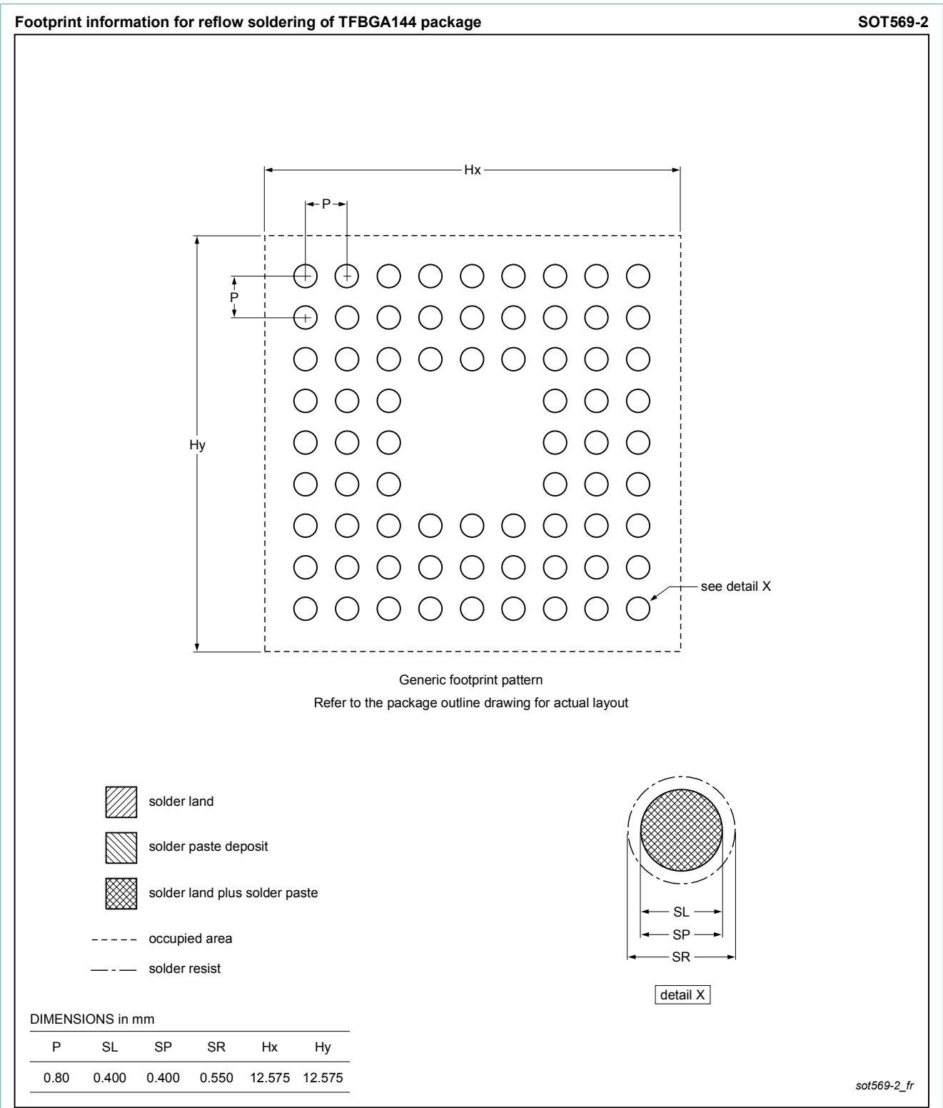
Fig. 2. Reflow soldering footprint for TFBGA144 (SOT569-2)
