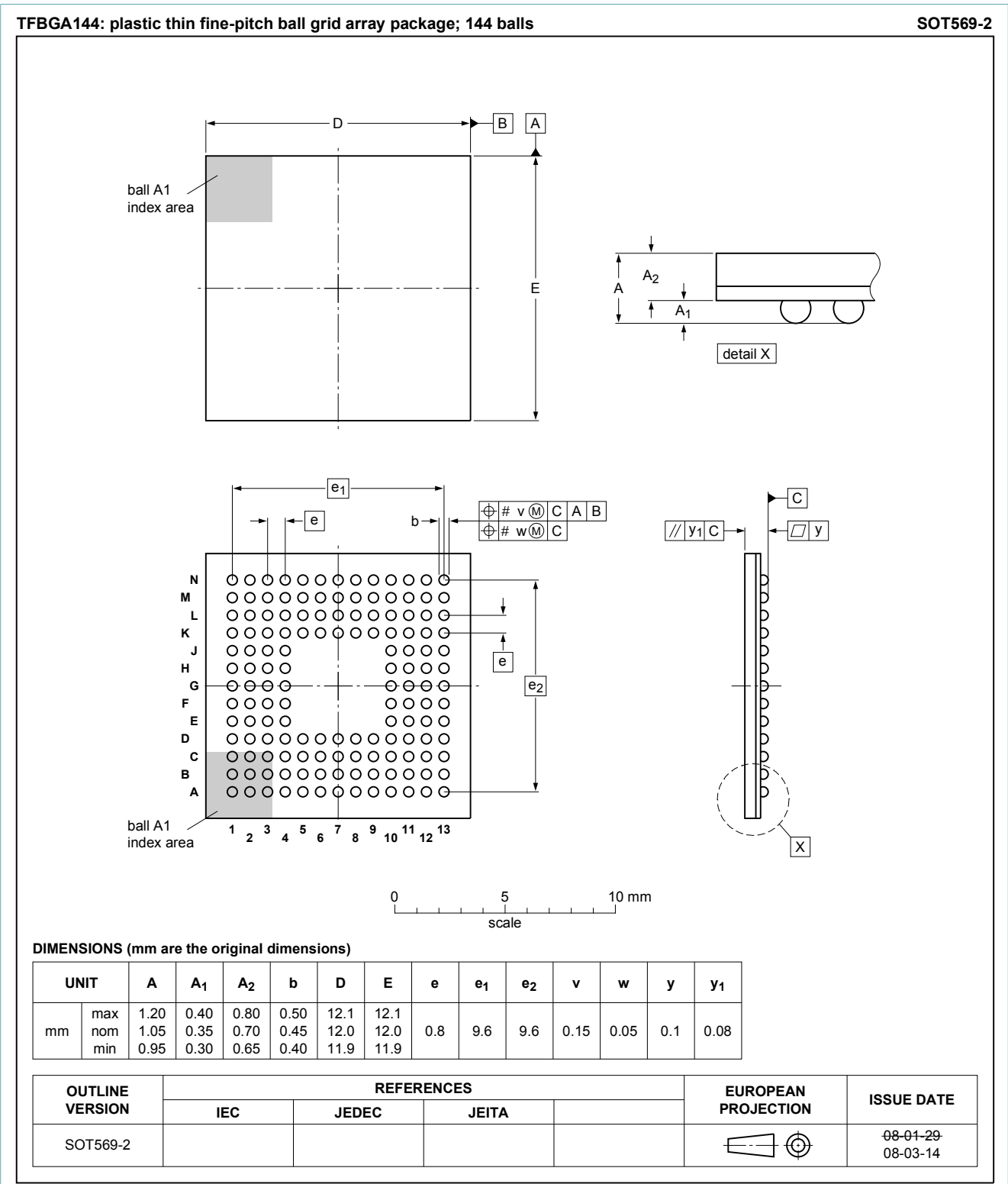
Fig. 1. Package outline TFBGA144 (SOT569-2)
