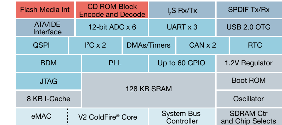
ColdFire® MCF5251 Block Diagram
