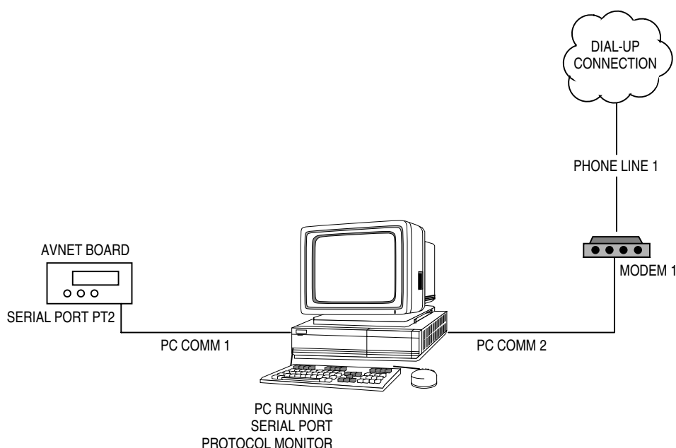
Figure 17. Serial Data Stream Monitor Tool Configuration
