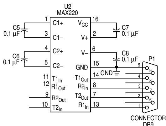
Figure 2. AN2120/D Serial Port Schematic
