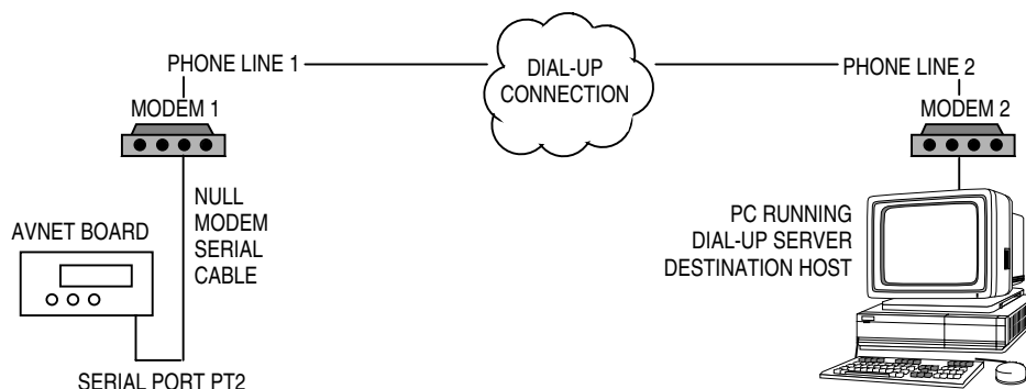
Figure 6. Demo Device Setup
