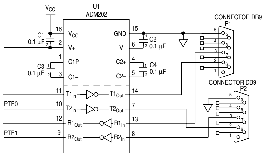
Figure 3. Avnet Serial Ports Schematic
