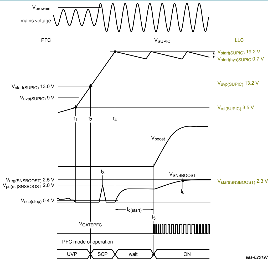
Figure 4. Start-up of the PFC and LLC
