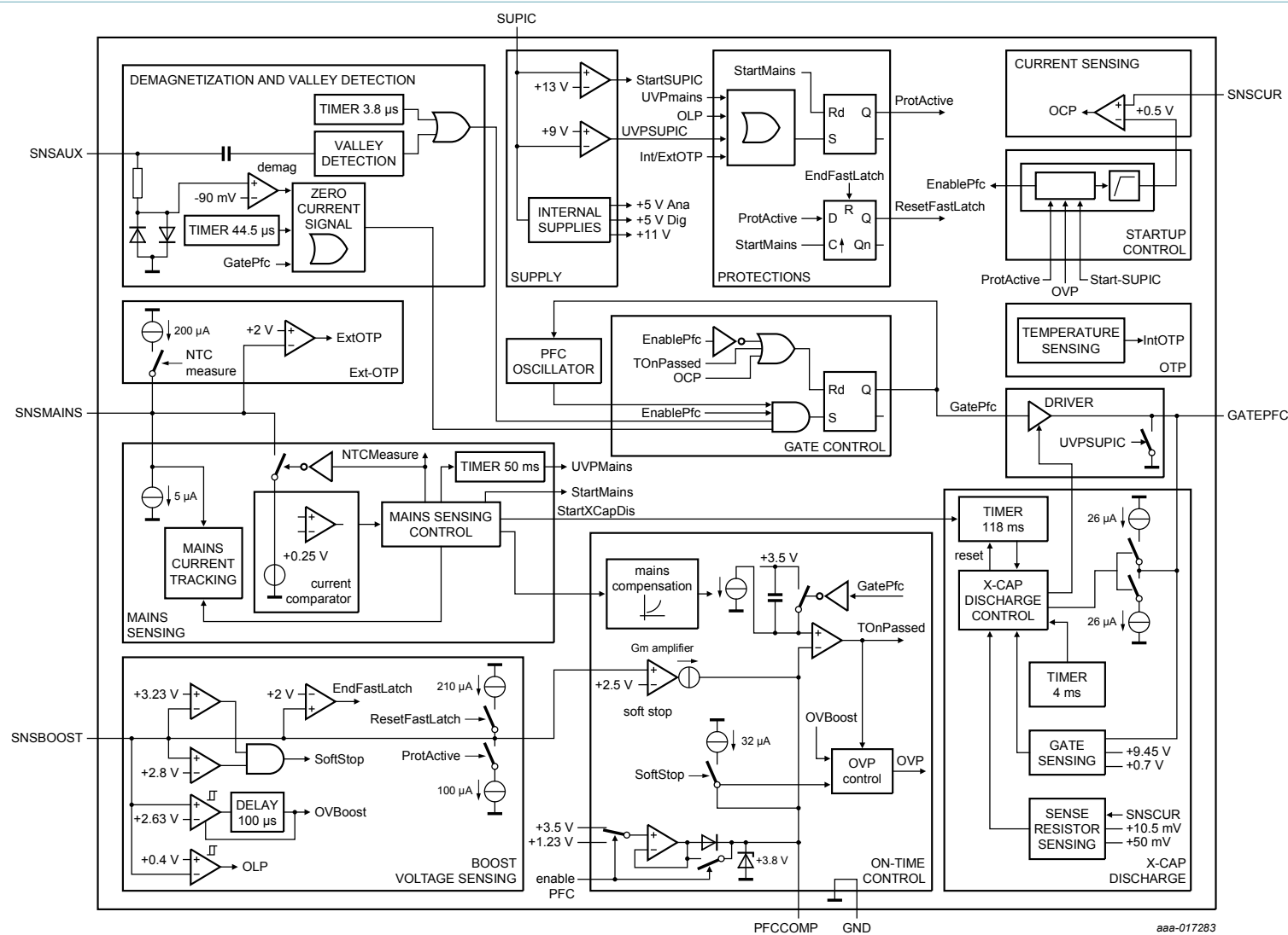
Figure 1. Block diagram
