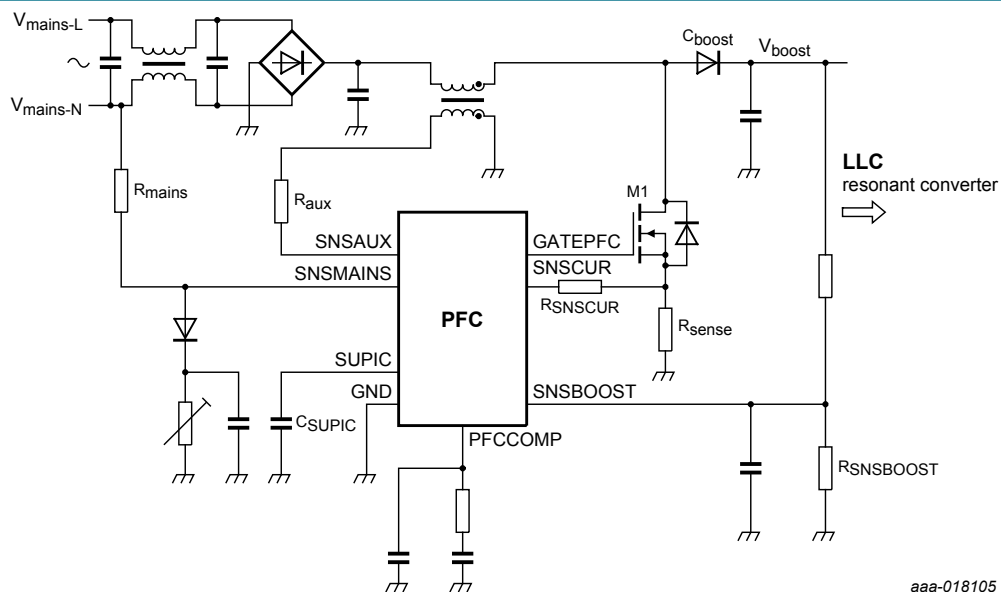
Figure 13. Application diagram
