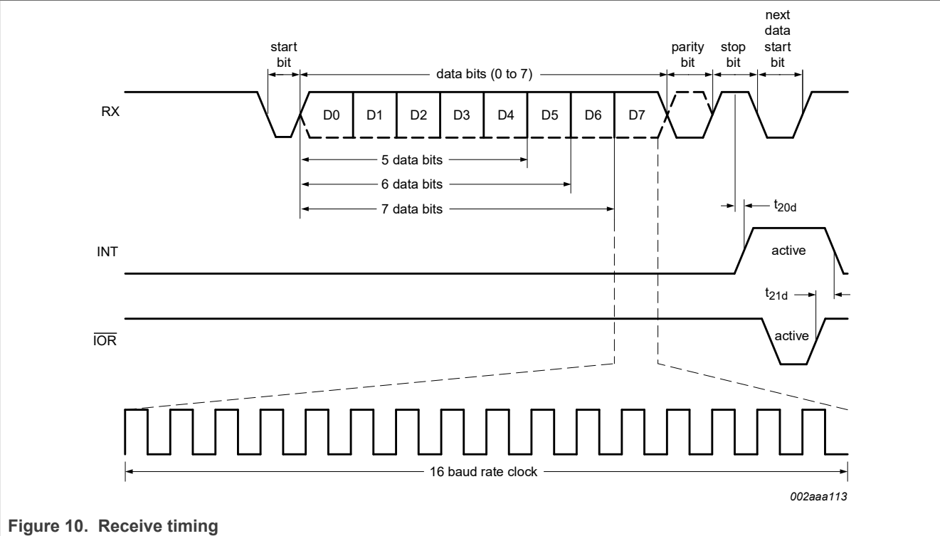
Figure 10. Receive timing
