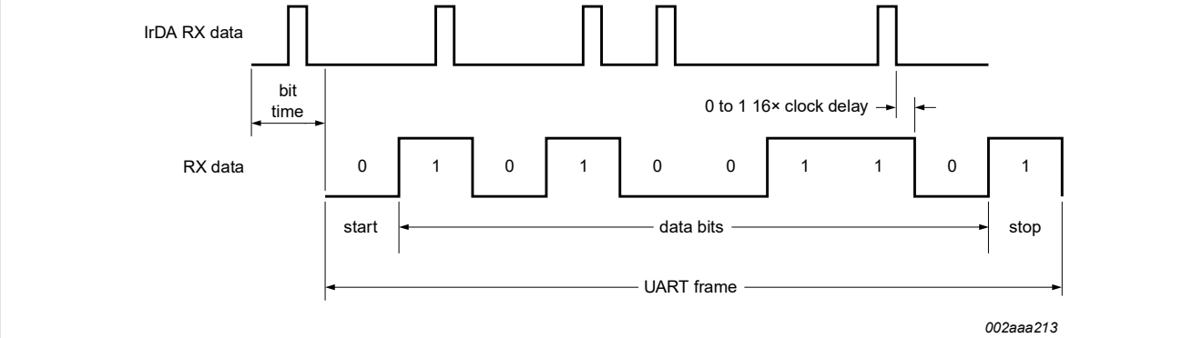
Figure 17. Infrared receive timing
