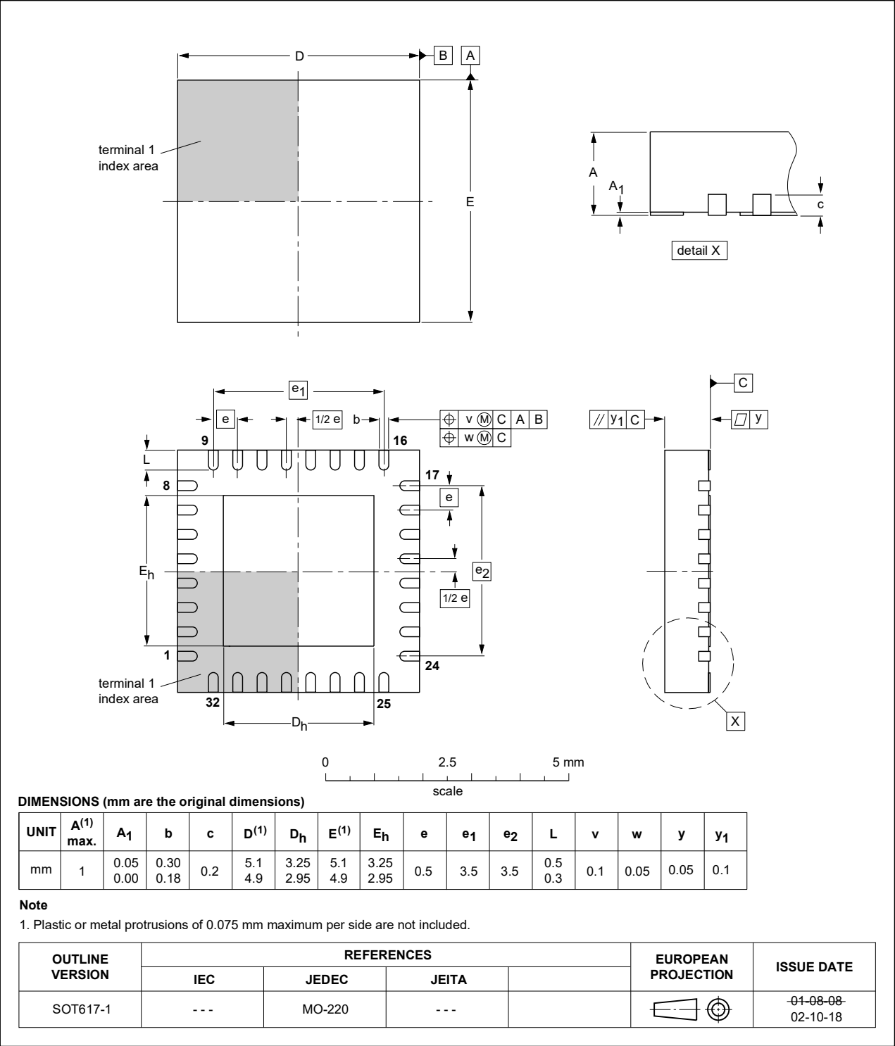
Figure 19. Package outline SOT617-1 (HVQFN32)
