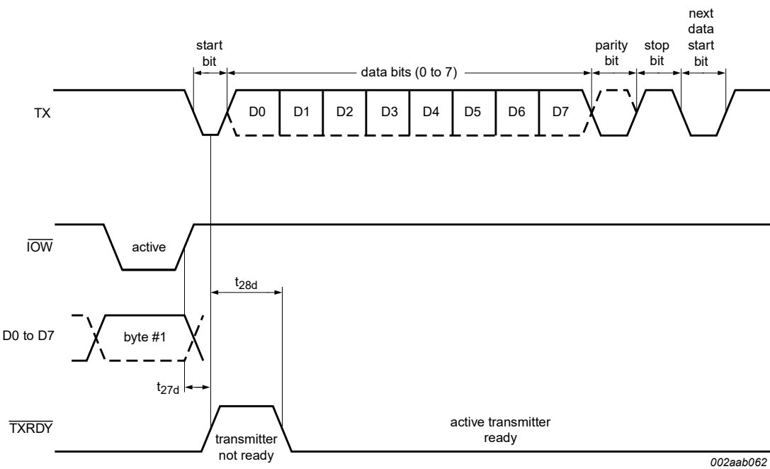
Figure 14. Transmit ready timing in non-FIFO mode
