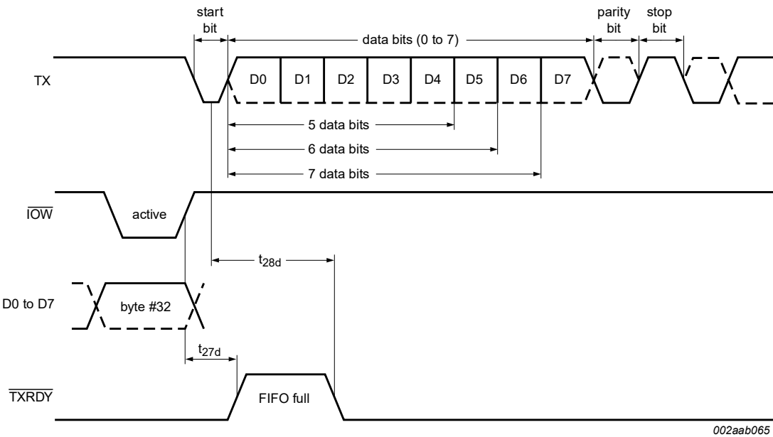
Figure 15. Transmit ready timing in FIFO mode (DMA mode '1')
