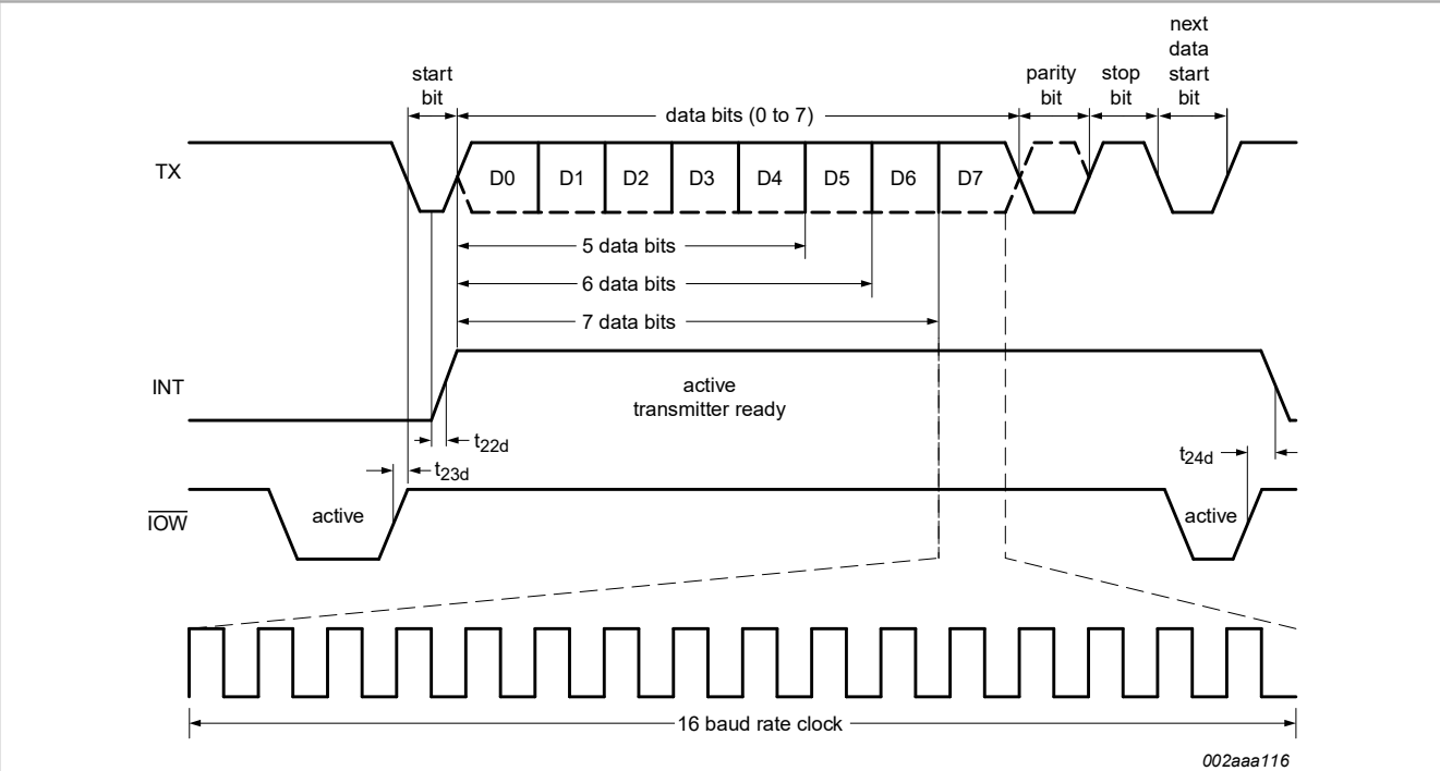
Figure 13. Transmit timing
