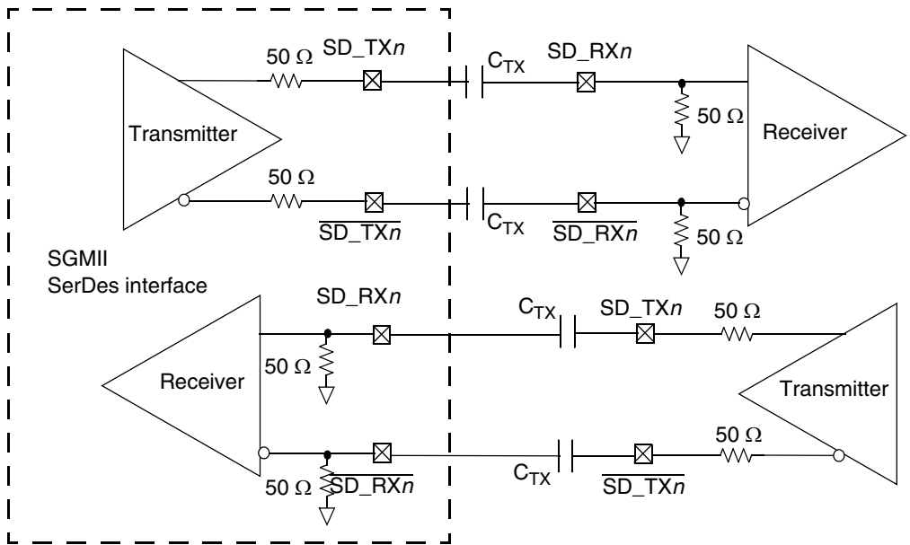
Figure 46. 4-wire, AC-coupled, SGMII serial link connection example
