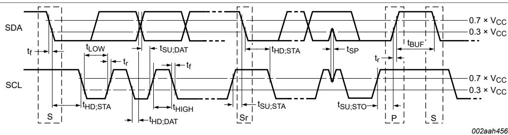
Figure 29. Timing diagram
