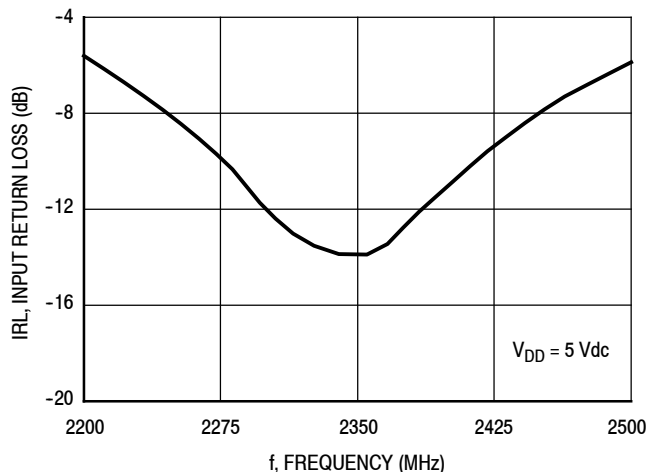
Figure 30. Input Return Loss (S11) versus Frequency
