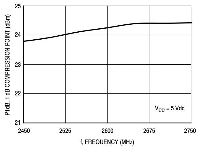
Figure 40. P1dB versus Frequency
