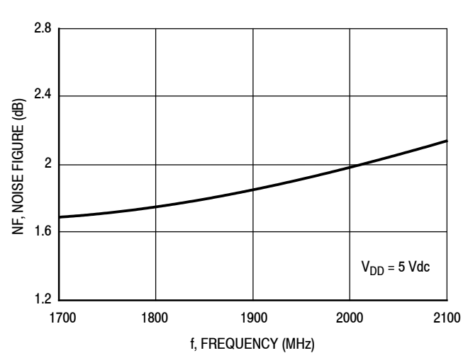
Figure 26. Noise Figure versus Frequency
