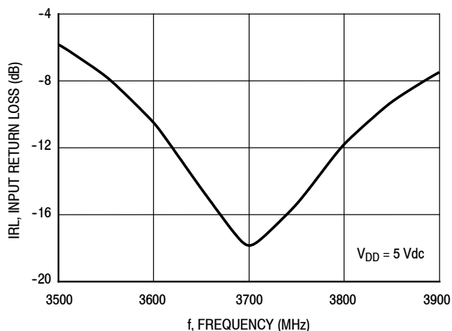
Figure 46. Input Return Loss (S11) versus Frequency
