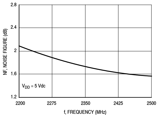
Figure 34. Noise Figure versus Frequency
