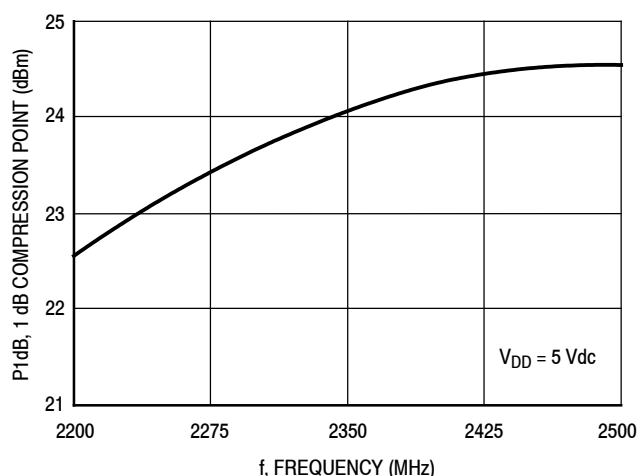
Figure 32. P1dB versus Frequency
