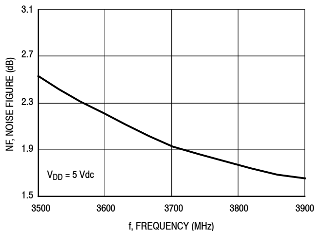
Figure 50. Noise Figure versus Frequency
