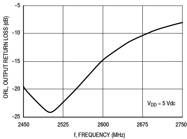
Figure 39. Output Return Loss (S22) versus Frequency
