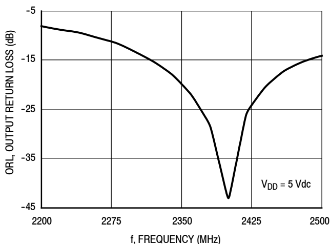
Figure 31. Output Return Loss (S22) versus Frequency
