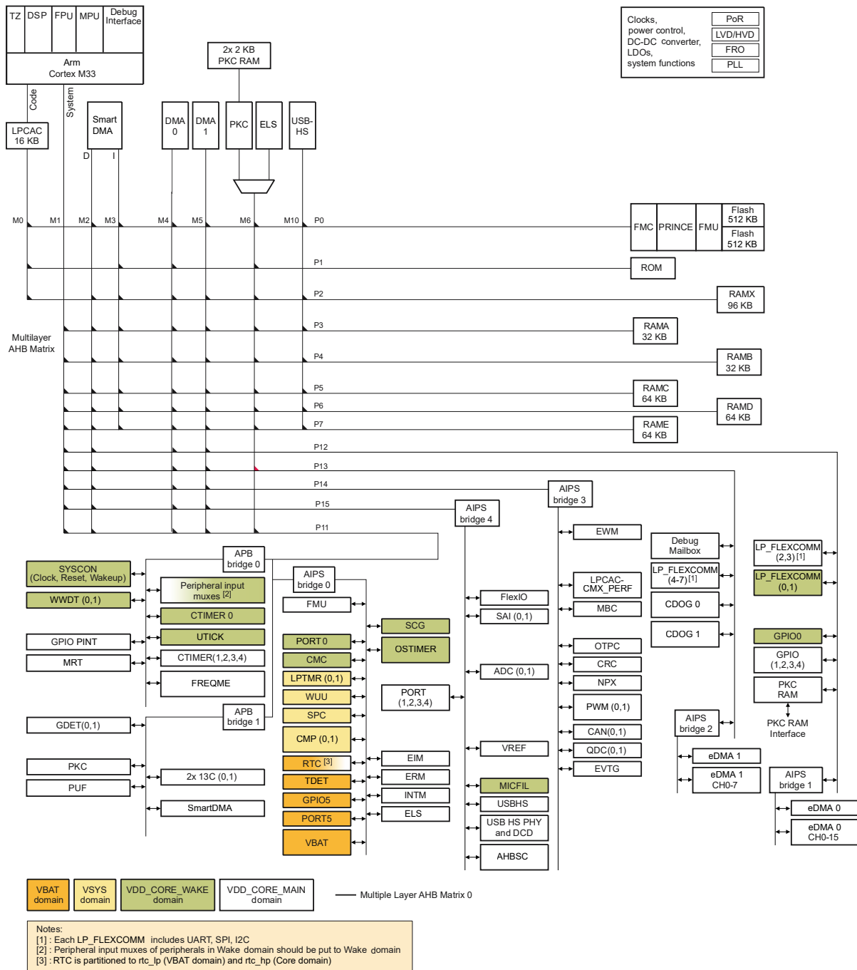
Figure 2. MCXN23x Architecture
