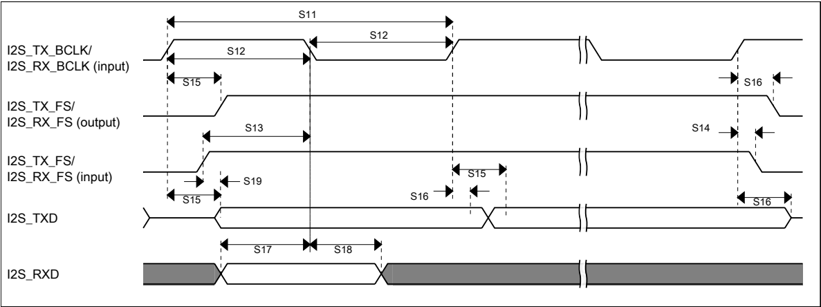
Figure 26. I2S/SAI timing — slave modes
