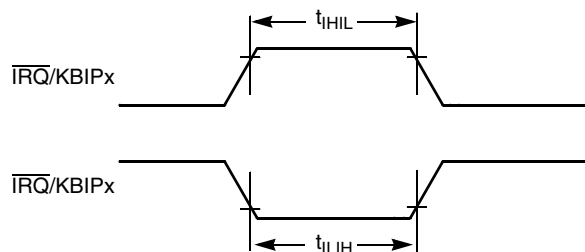
Figure 20. \overline{\text{IRQ}}/\text{KBIPx} Timing
