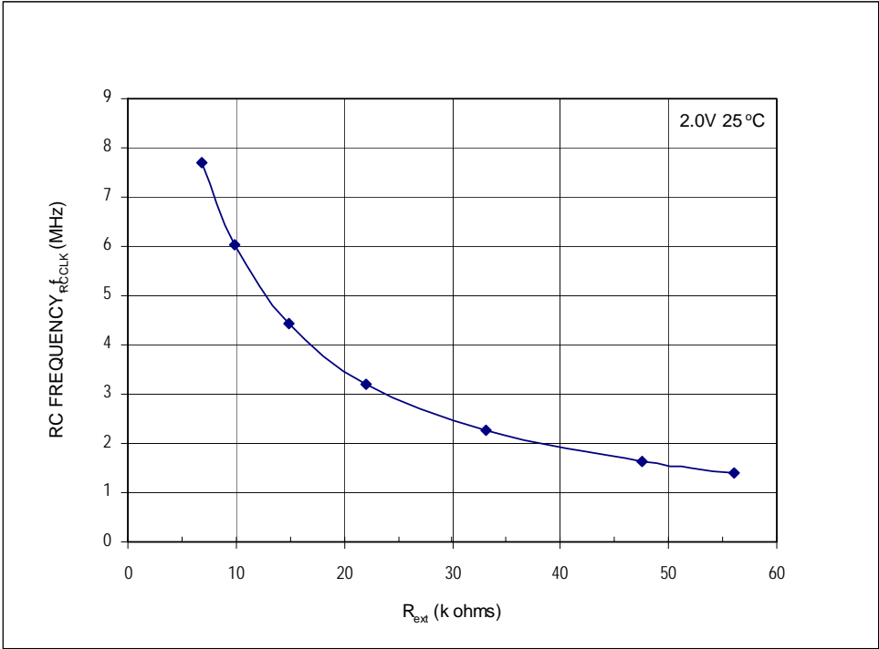
Figure 16-12. RC versus Frequency (2 Volts @ 25°C)
