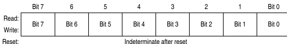
Figure 14-13. TIM Channel x Register Low (TCHxL)
