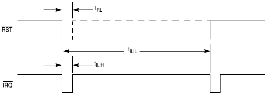
Figure 16-9. \overline{RST} and \overline{IRQ} Timing
