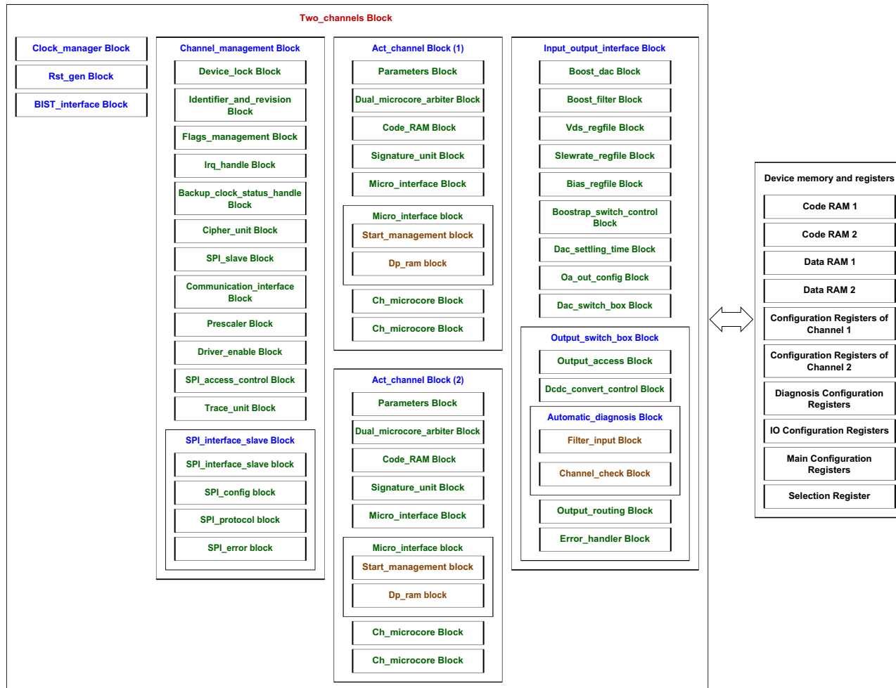
Figure 26. Device logic block hierarchic overview
