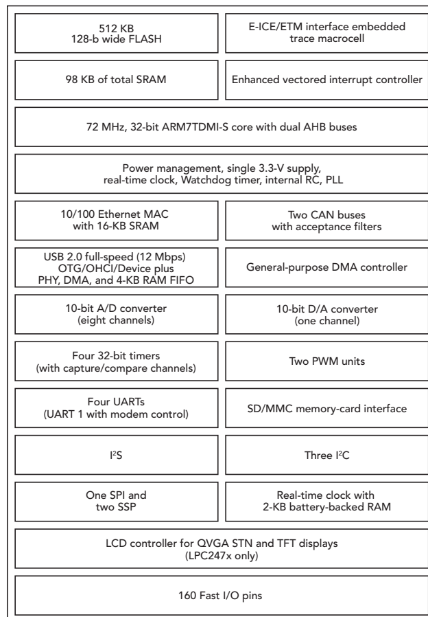
LPC24xx block diagram
