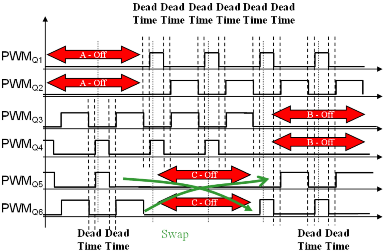
Figure 2-5. Bipolar PWM switching — detail
