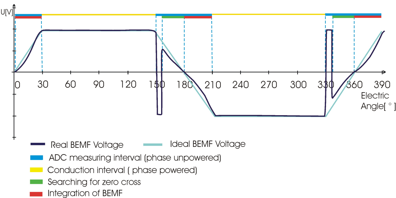
Figure 2-8. Single phase voltage waveform
