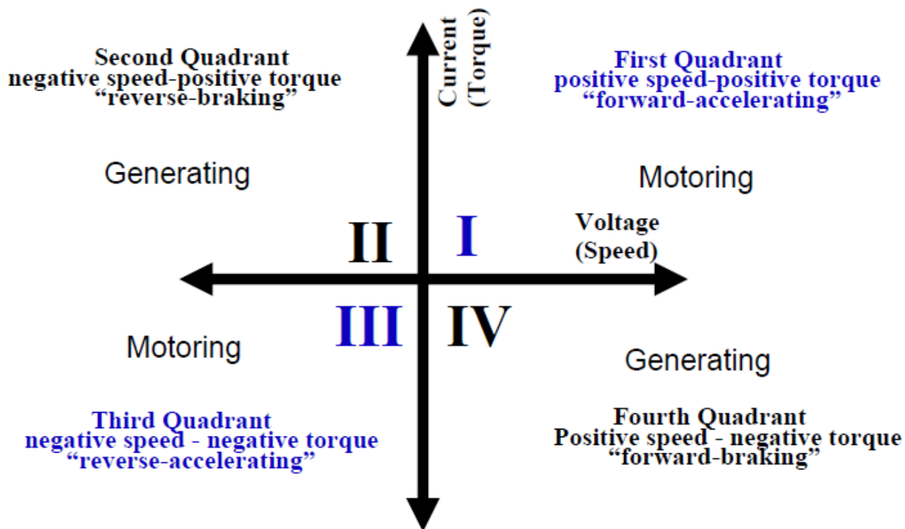
Figure 2-6. The 4-quadrant operation
