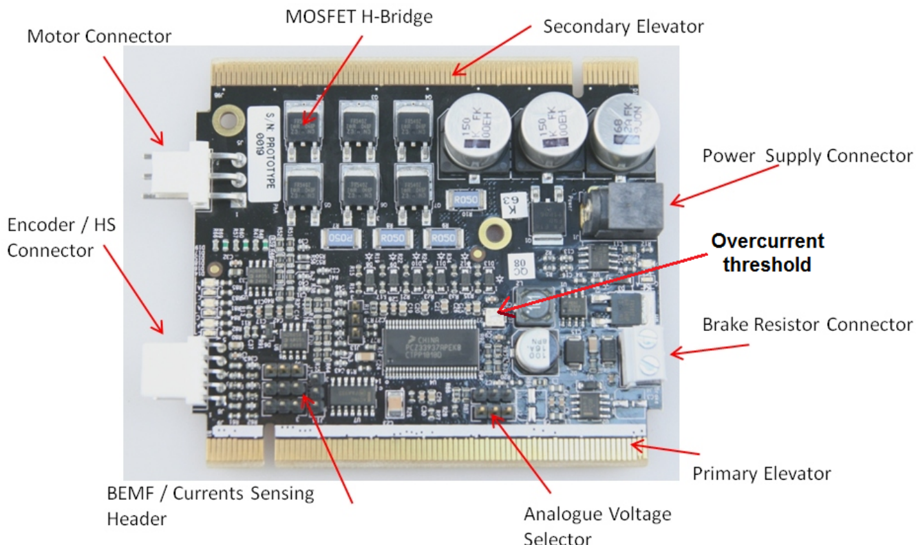
Figure 5-2. TWR-MC-LV3PH Image
