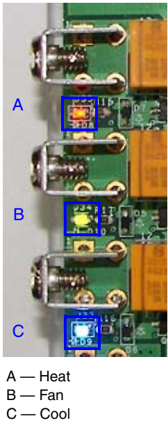
Figure 2-7. LEDs location
