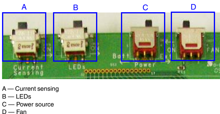
Figure 2-5. Thermostat switches
