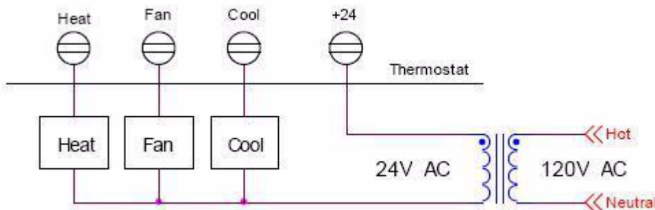
Figure 2-1. Configuration diagram
