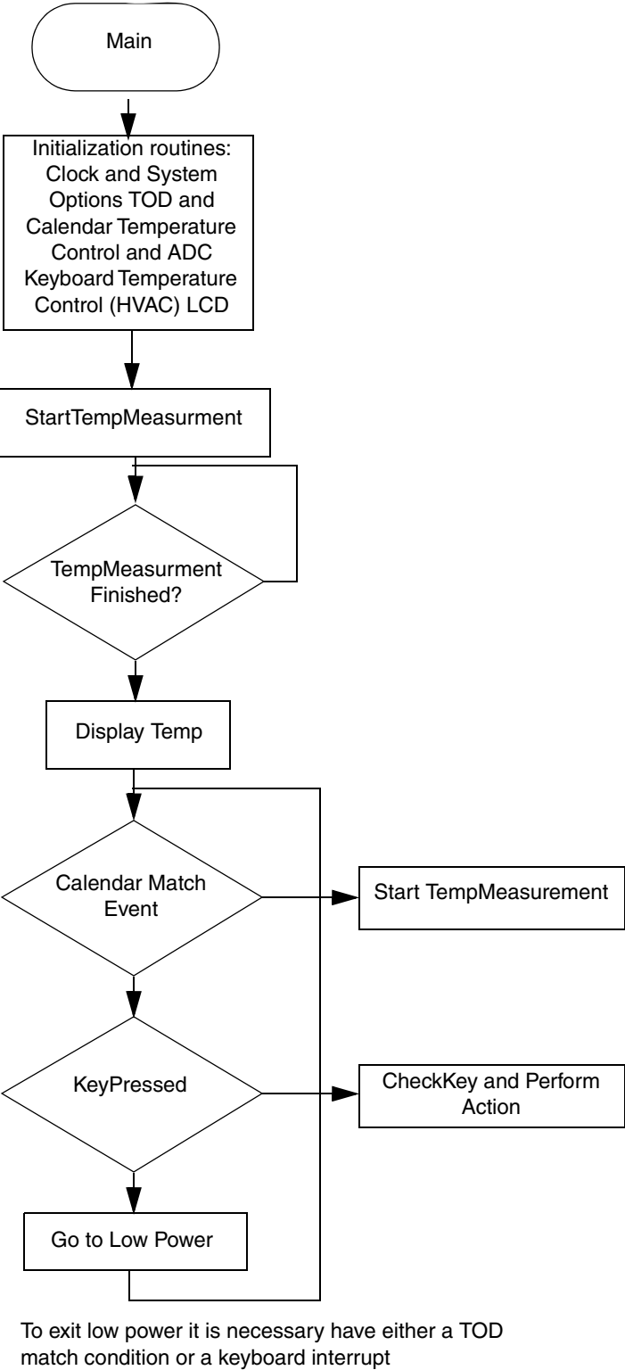
Figure 3-1. High level thermostat workflow flow diagram
