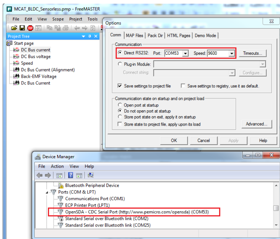
Figure 4. FreeMASTER settings
