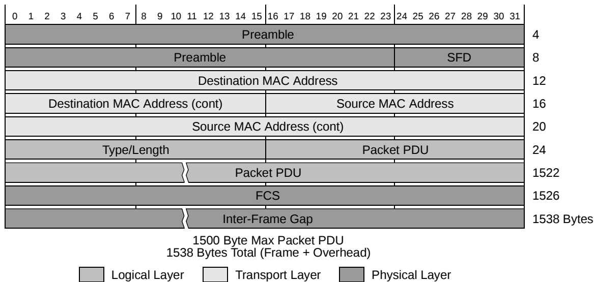
Figure 5. Layer 2 Ethernet Packet Format
