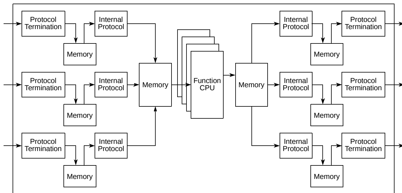
Figure 1. Generic Embedded Communications System
