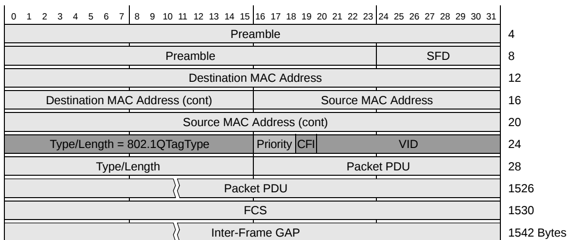
Figure 8. Layer 2 VLAN Tag
