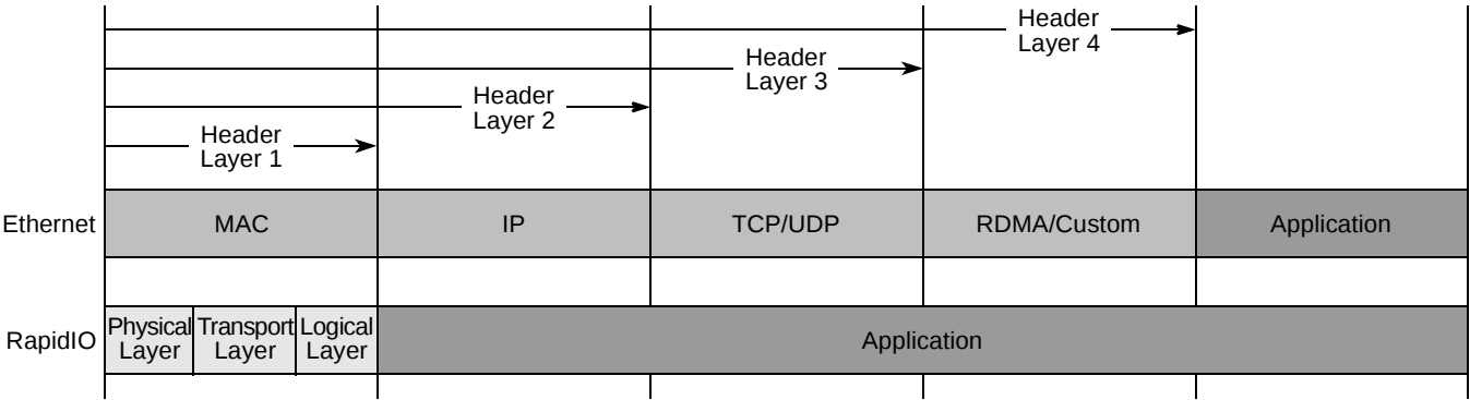
Figure 12. Header Layering
