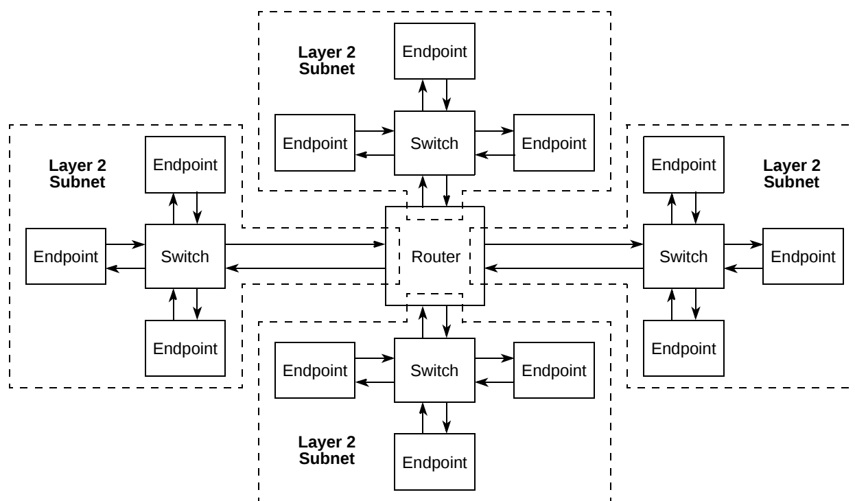
Figure 7. IP Network
