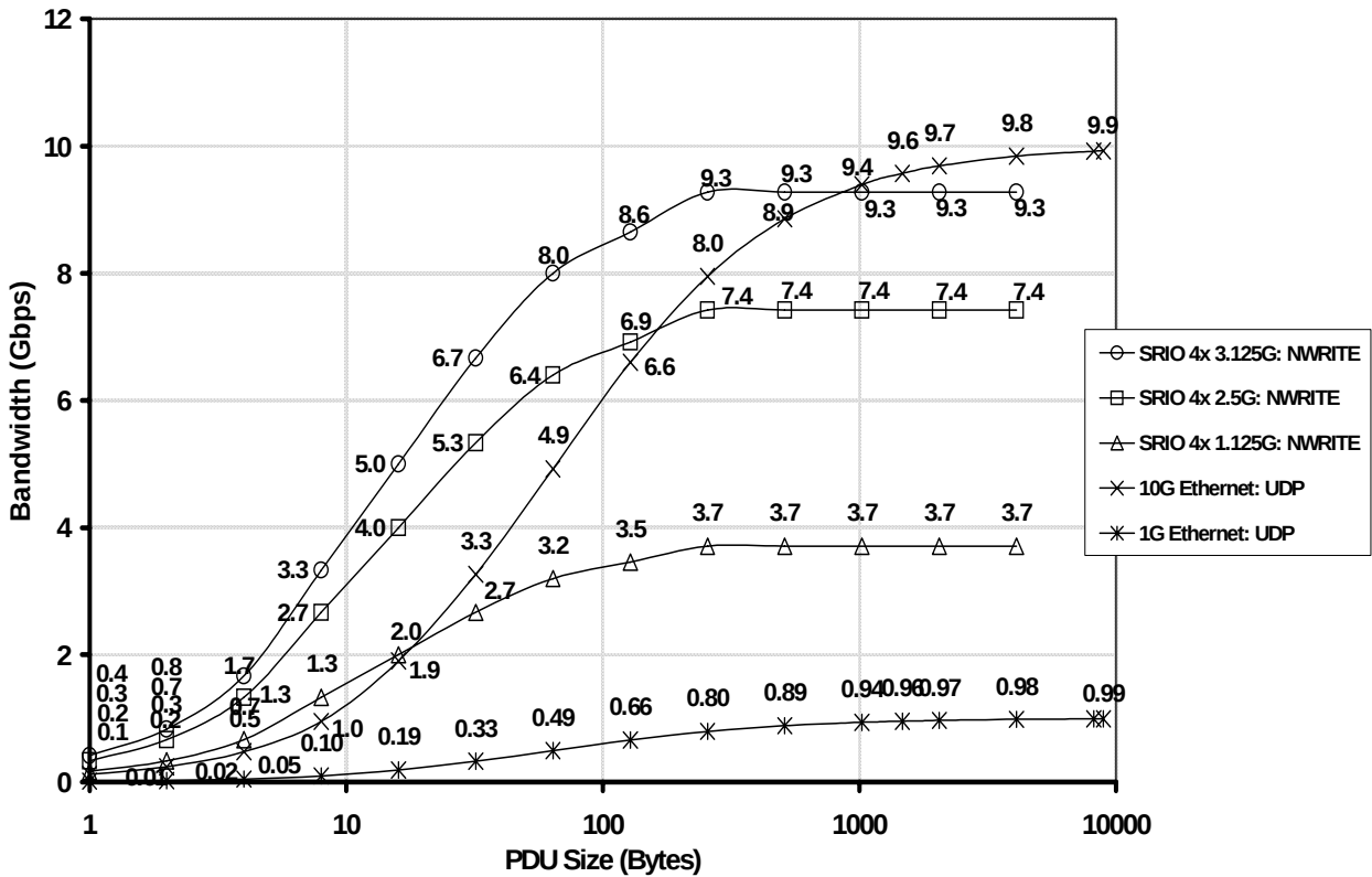
Figure 14. Effective Bandwidth
