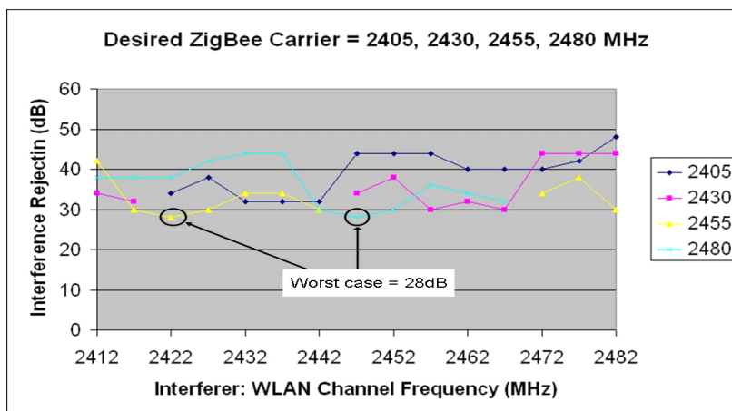
Figure 22. Worst Case Results (WLAN Interferers)
