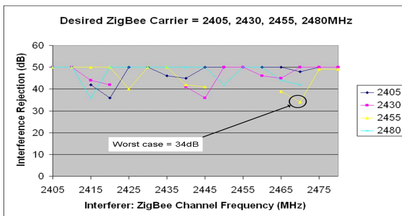
Figure 21. Worst Case Results (Zigbee Interferers)
