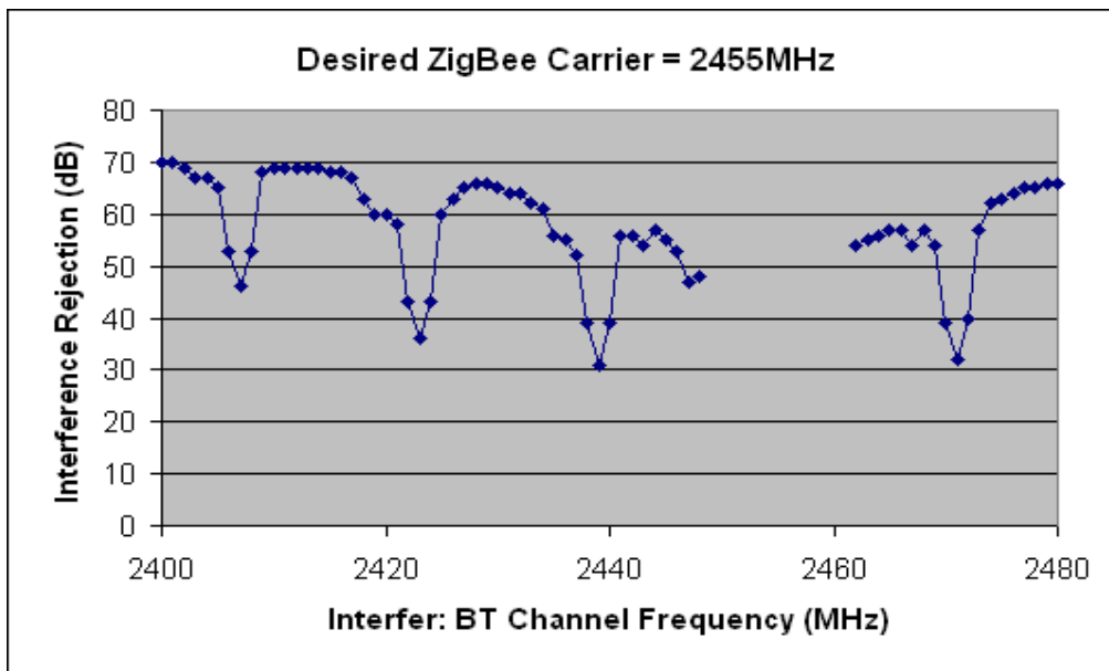
Figure 19. Desired ZigBee Carrier = 2455MHz (BlueTooth Interferer)
