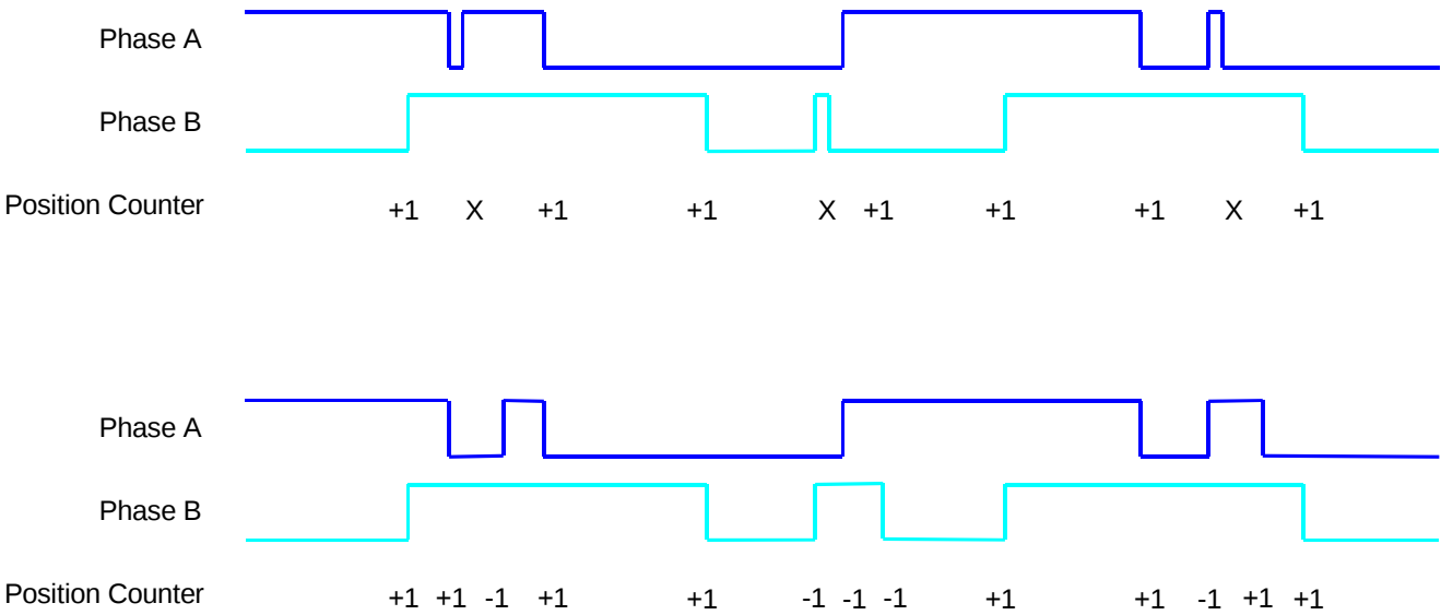
Figure 5. Noise immunity
