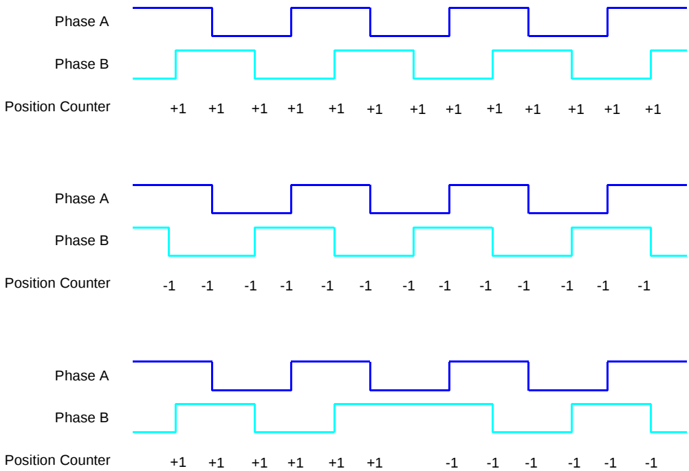
Figure 2. 32-bit Linear Quadrature Decoder
