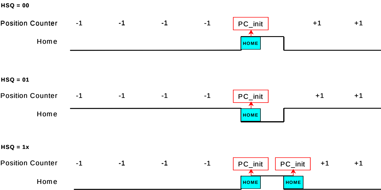
Figure 6. 32LQD_home timing
