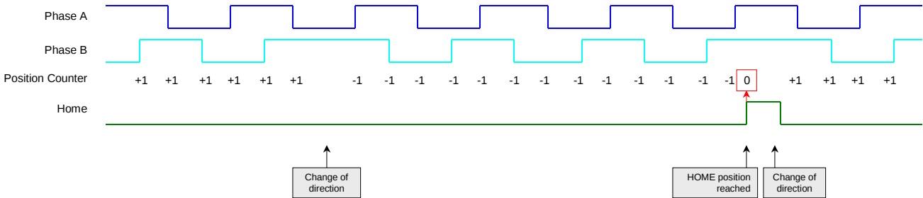
Figure 1. Signals processed by 32LQD TPU function set and corresponding PC value
