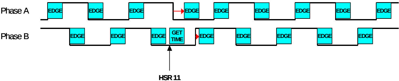
Figure 3. 32LQD timing
