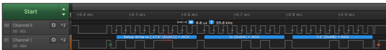
Figure 6. Reading two bytes from slave device with 0x56 address
