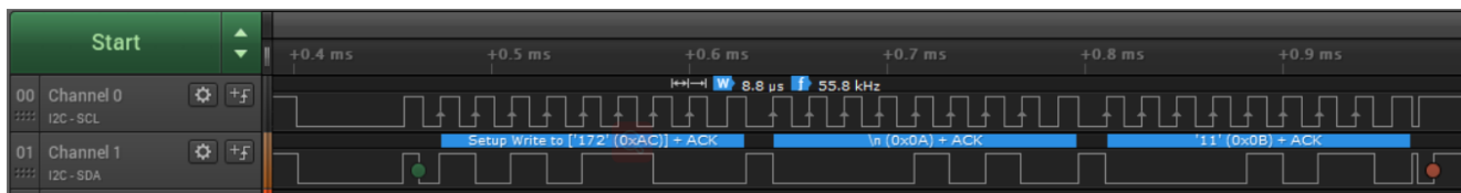
Figure 5. Write two bytes to slave device with 0x56 address
