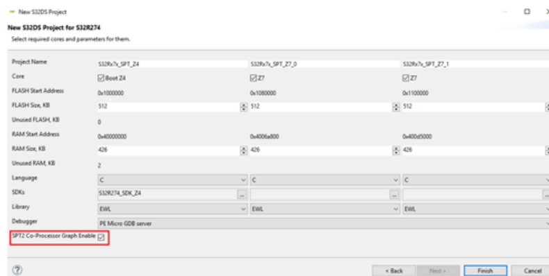
Figure 6. Generate project with SPT graphical tool
