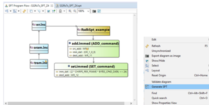
Figure 8. Example working flow and generate code
