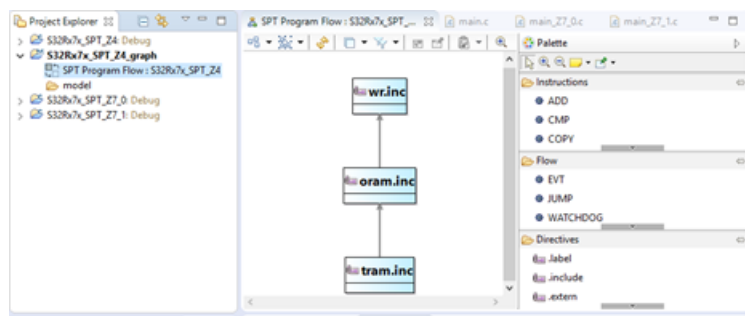
Figure 7. SPT graphical tool windows
