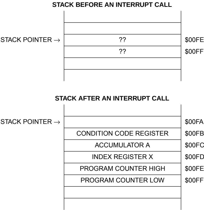
Figure 2. Stack Before and After an Interrupt Call
