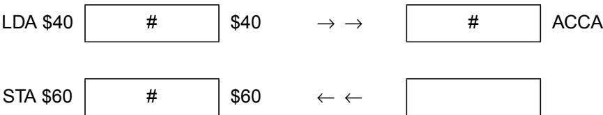
Figure 7. Accumulator as a Bottleneck
