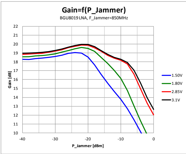
Fig 10. Gain versus jammer power at 850 MHz
