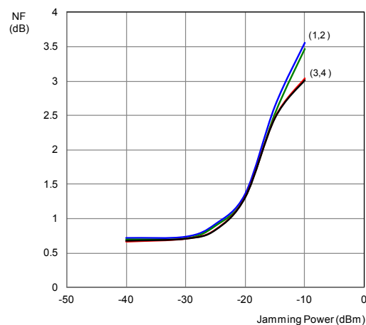
f_{jam} = 1850\text{ MHz} ; T_{amb} = 25\text{ }^{\circ}\text{C} ; f = 1575\text{ MHz} ; including PCB losses.
