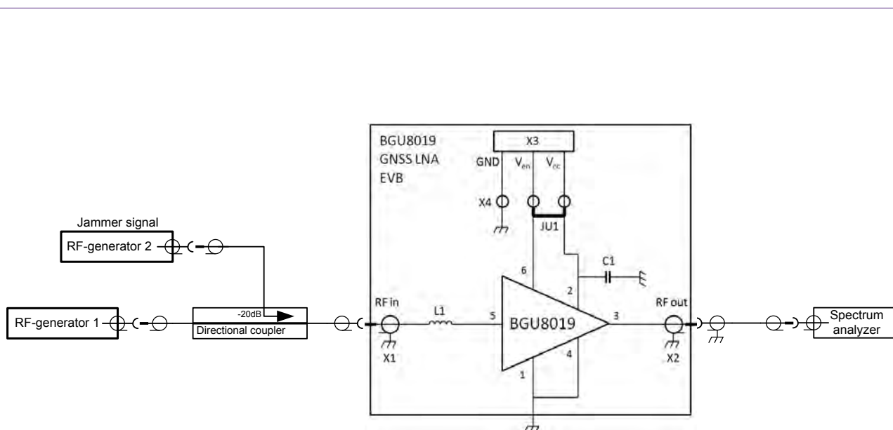
Fig 6. 1dB Gain compression under jamming measurement setup (LNA evaluation board)
