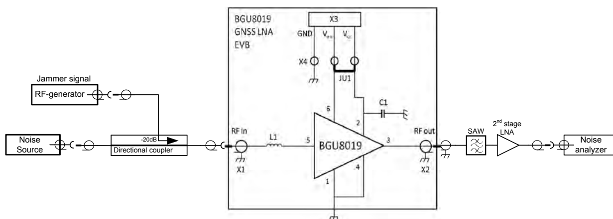
Fig 13. Noise under jamming measurement setup (LNA evaluation board)
