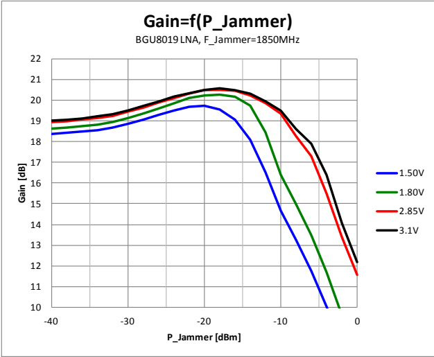
Fig 12. Gain versus jammer power at 1850 MHz
