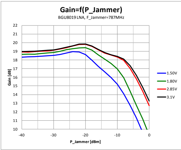
Fig 8. Gain versus jammer power at 787 MHz
