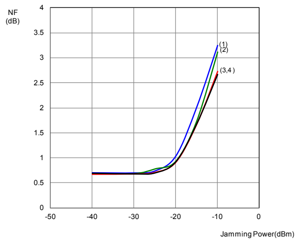
f_{jam} = 850\text{ MHz} ; T_{amb} = 25\text{ }^{\circ}\text{C} ; f = 1575\text{ MHz} ; including PCB losses.
